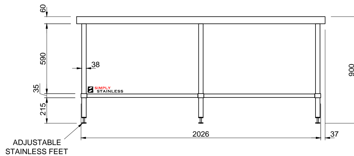
FRONT ELEVATION
