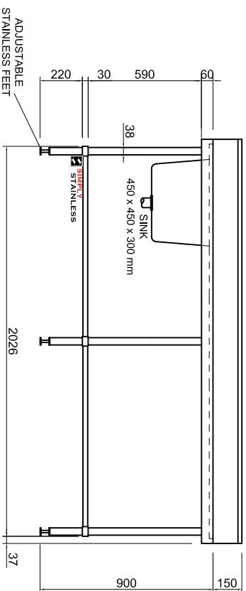
FRONT ELEVATION
