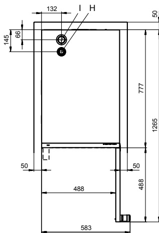
View from above with wall clearances
