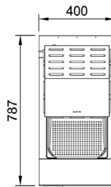
Plan View
