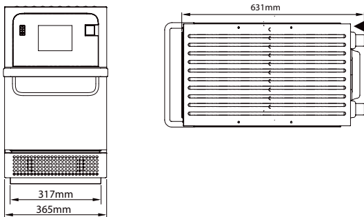
Internal cavity width 311mm
