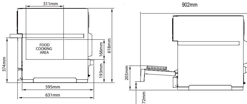
Internal cavity width 311mm
